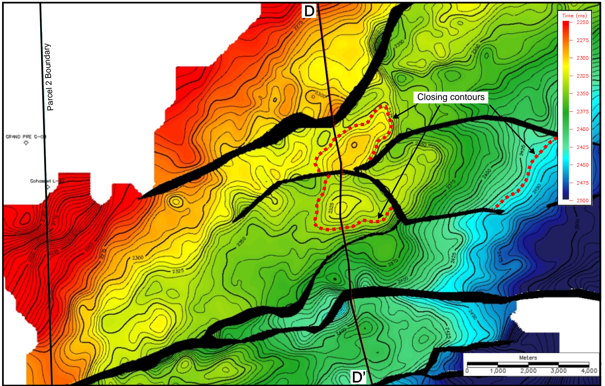
Structure map of a lower Mississauga seismic marker showing the Propeller prospect and the location of seismic profile D-D'.
